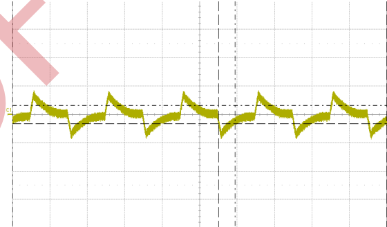
Fig. 12: Output voltage response to load current step-change (10 A – 15 A – 10 A) at V_{in} = 48 V. Current slew rate: 0.1 A/ \mu s. C_o = 4700 \mu F E-cap + 1 \mu F ceramic + 10 \mu F tantalum. Time scale: 500 \mu s/div.
