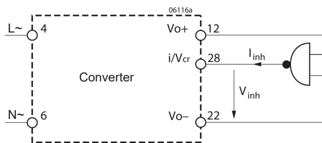
Fig. 14 Inhibit connection
