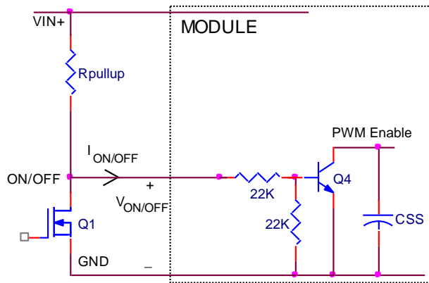
Figure 40. Circuit configuration for using negative On/Off logic
