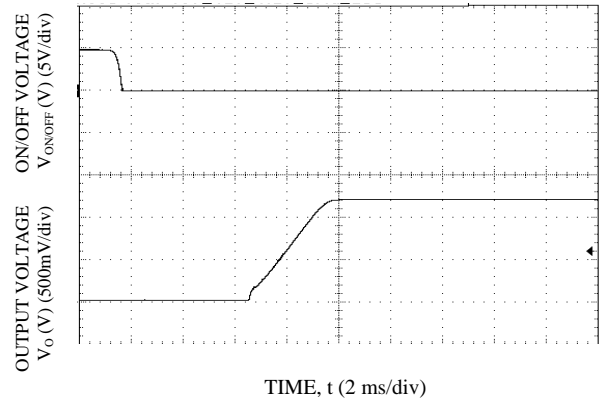
Figure 26. Start-up Using On/Off Voltage ( I_O = I_{O,max} ), V_O = 1.2\text{ V}
