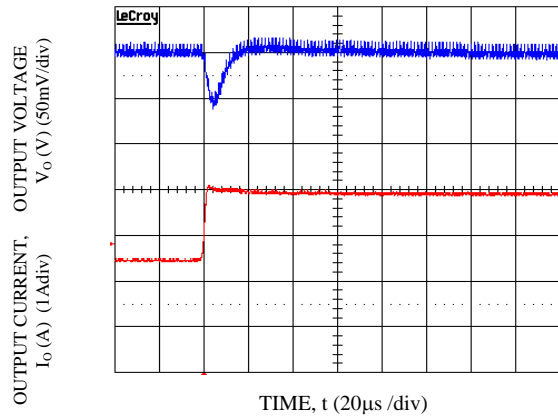
Figure 23. Transient Response to Dynamic Load Change from 50% to 100% at 12 Vin, Cout=2x47 \mu F, CTune=2200 pF & RTune=261 \Omega . Vo = 3.3 V
