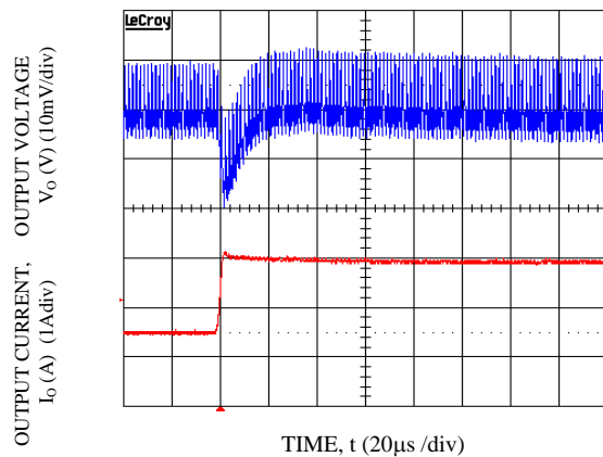
Figure 21. Transient Response to Dynamic Load Change from 50% to 100% at 12 Vin, Cout-1x47 \mu F+1x330 \mu F, CTune-10 nF & RTune-261 \Omega . V_o = 1.8 V
