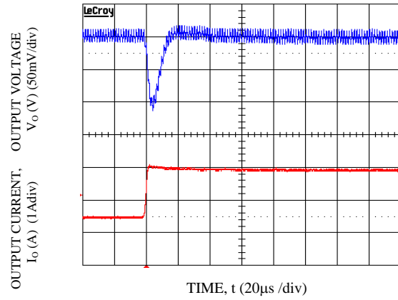
Figure 24. Transient Response to Dynamic Load Change from 50% to 100% at 12 Vin, Cout=1x47 \mu F, CTune=820 pF & RTune=261 \Omega . Vo = 5 V
