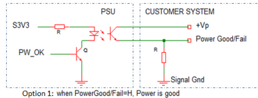
Option 1: when PowerGood/Fail=H, Power is good
