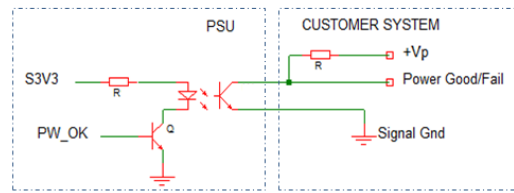
Option 2: when PowerGood/Fail=L, Power is good
