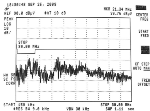
Figure 8 – Conducted Noise
