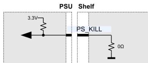
Figure 18. PS_KILL connection
