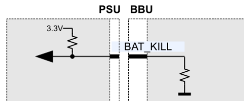
Figure 19. BAT_KILL connection
