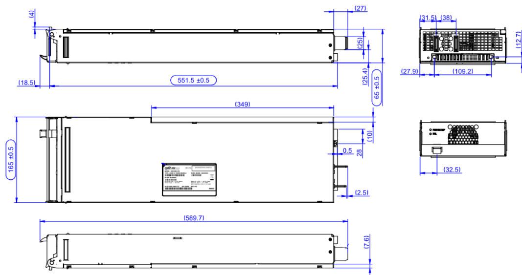
Figure 24. Mechanical Drawing
