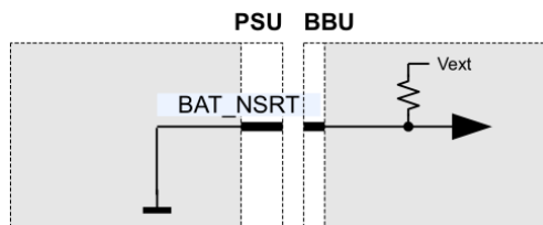
Figure 20. BAT_NSRT connection
