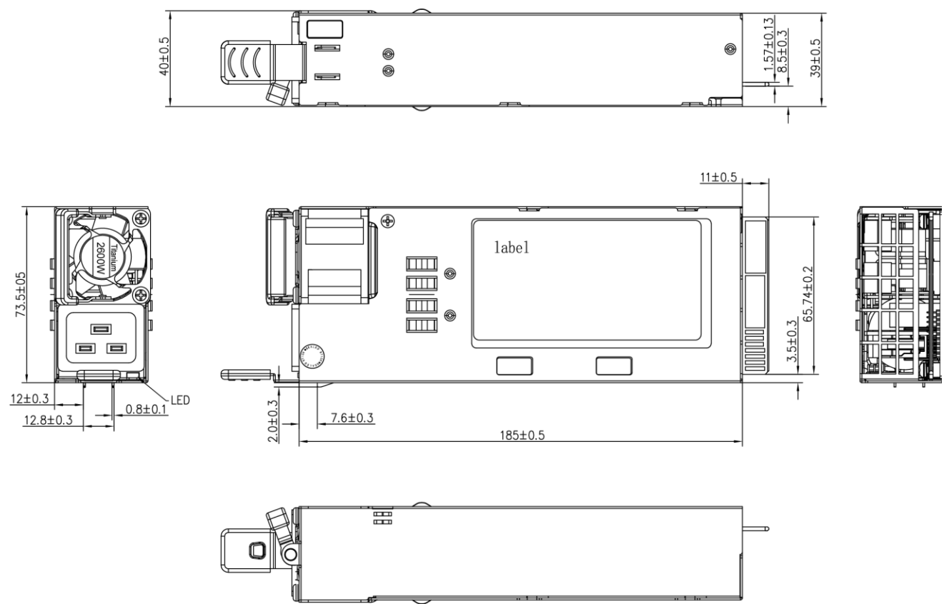
Figure 16. Mechanical Drawing
