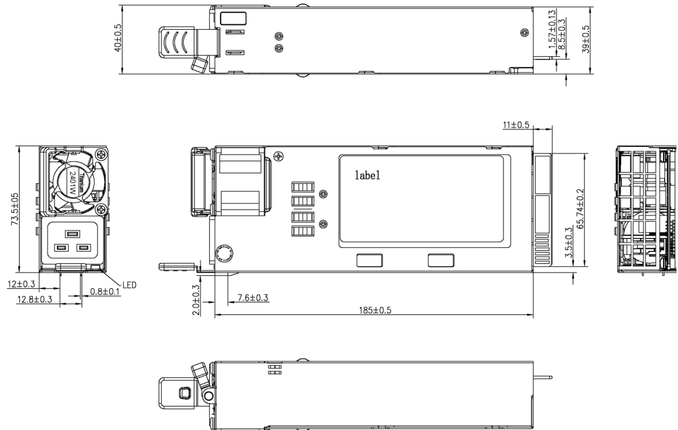
Figure 16. Mechanical Drawing
