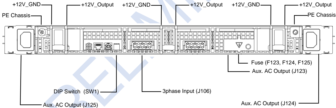
Figure 5. SPSPFE3-09 Rear View
