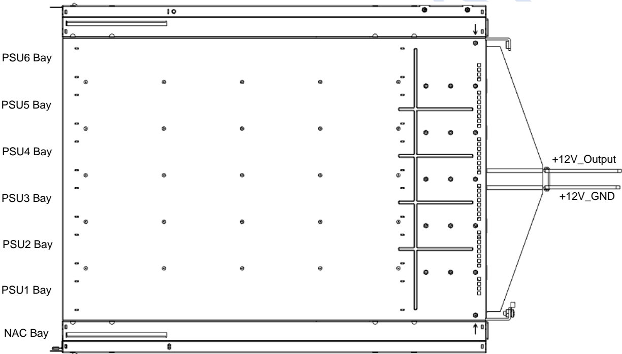
Figure 9. SPSPFE3-10 Top View
