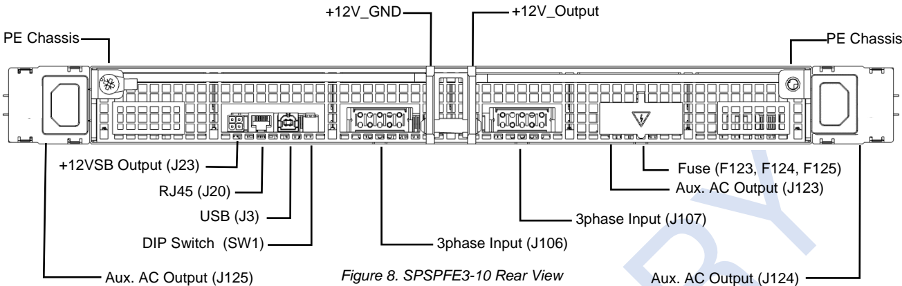
Figure 8. SPSPFE3-10 Rear View
