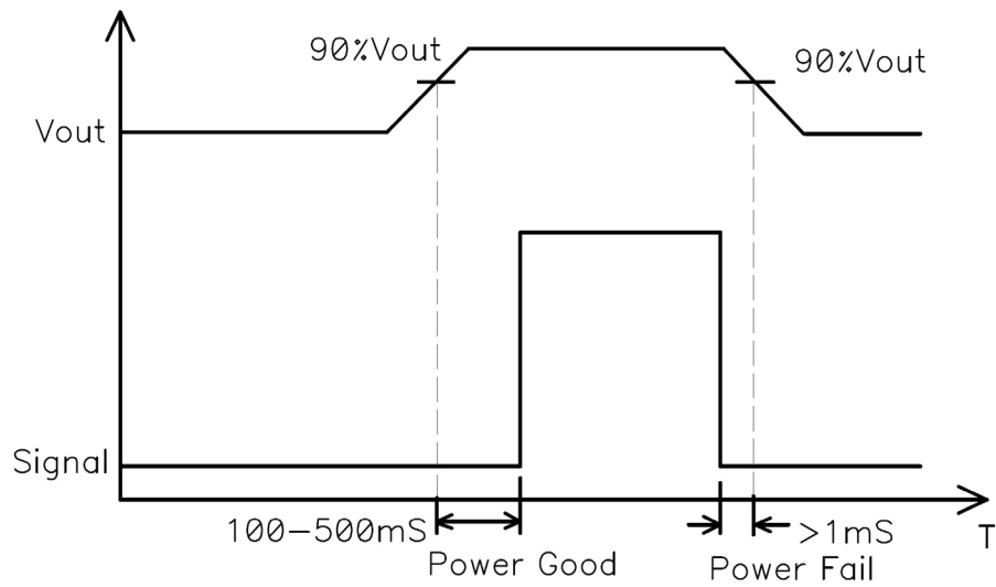
Figure 2. PG / PF signal diagram (available only for MEPG500-2XXX option)
