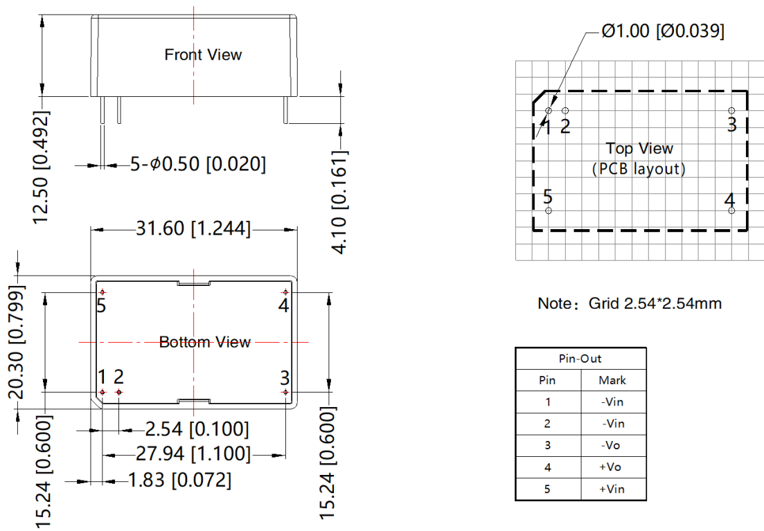
Figure 3. Mechanical drawing
