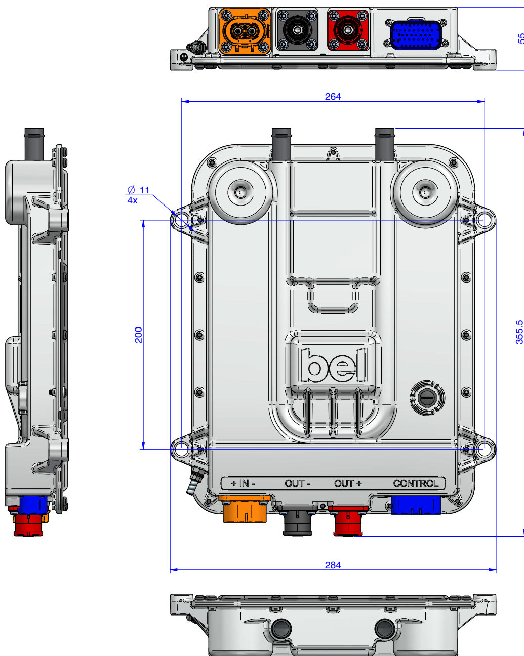
Figure 7. Mechanical Drawing
