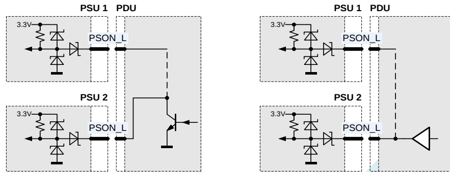
Figure 9. PSON_L connection
