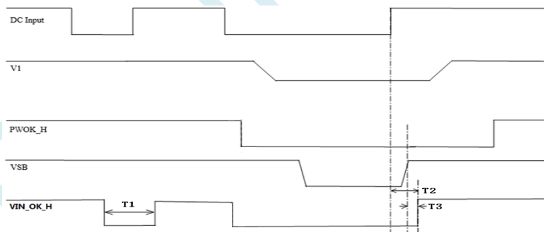
Figure 12. VIN_OK_H Timing
