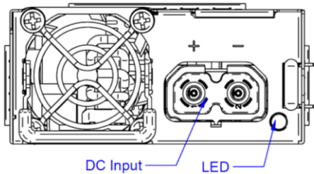
Figure 22. Front view
