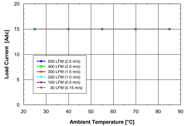
Fig. 1.5V.2: Available load current vs. ambient air temperature and airflow rates for SQ24T15015 converter mounted horizontally with B height pins with V_{in} = 24V , air flowing from pin 3 to pin 1 and maximum FET temperature \leq 120^{\circ}C .
