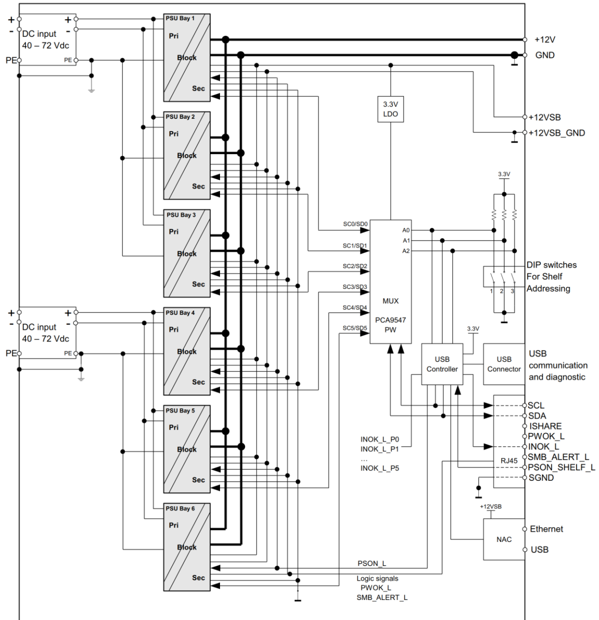
Figure 1. SPSFF3-0X Block Diagram
