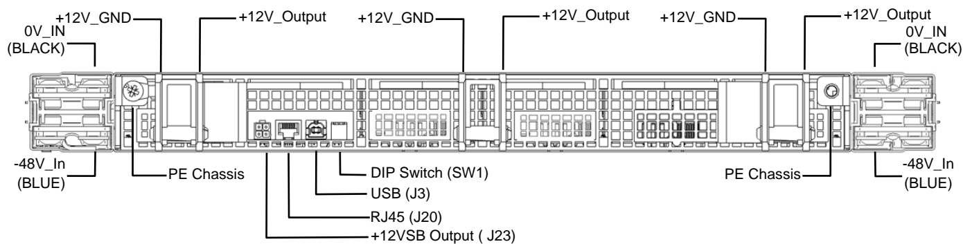
Figure 7. SPSPFF3-03 Rear View
