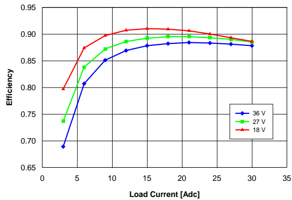
Figure 14. Efficiency vs. load current and input voltage for converter mounted horizontally with air flowing from pin 3 to pin 4 at a rate of 300 LFM (1.5 m/s) and T_a = 25^\circ\text{C} .
