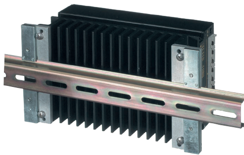
Fig. 29 DIN-rail mounting assembly HZZ00615-G (DMB-K/S)
