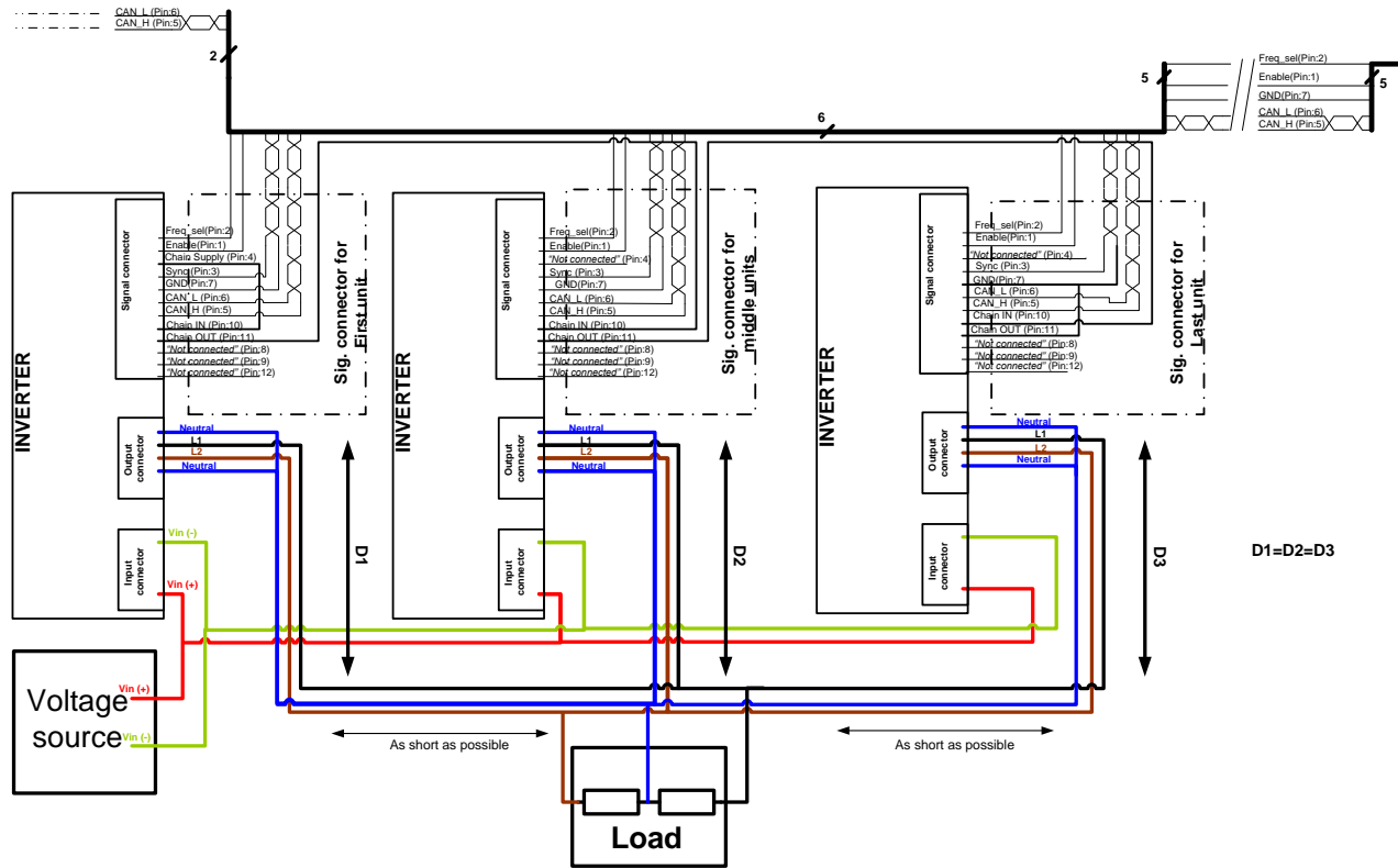
Wiring setup for parallel operation 700INV60-120-240-9G
