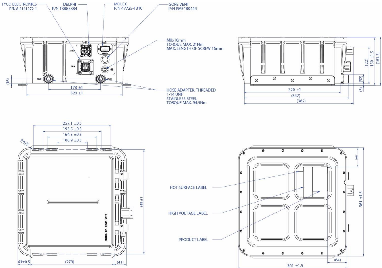
Mechanical Drawings
