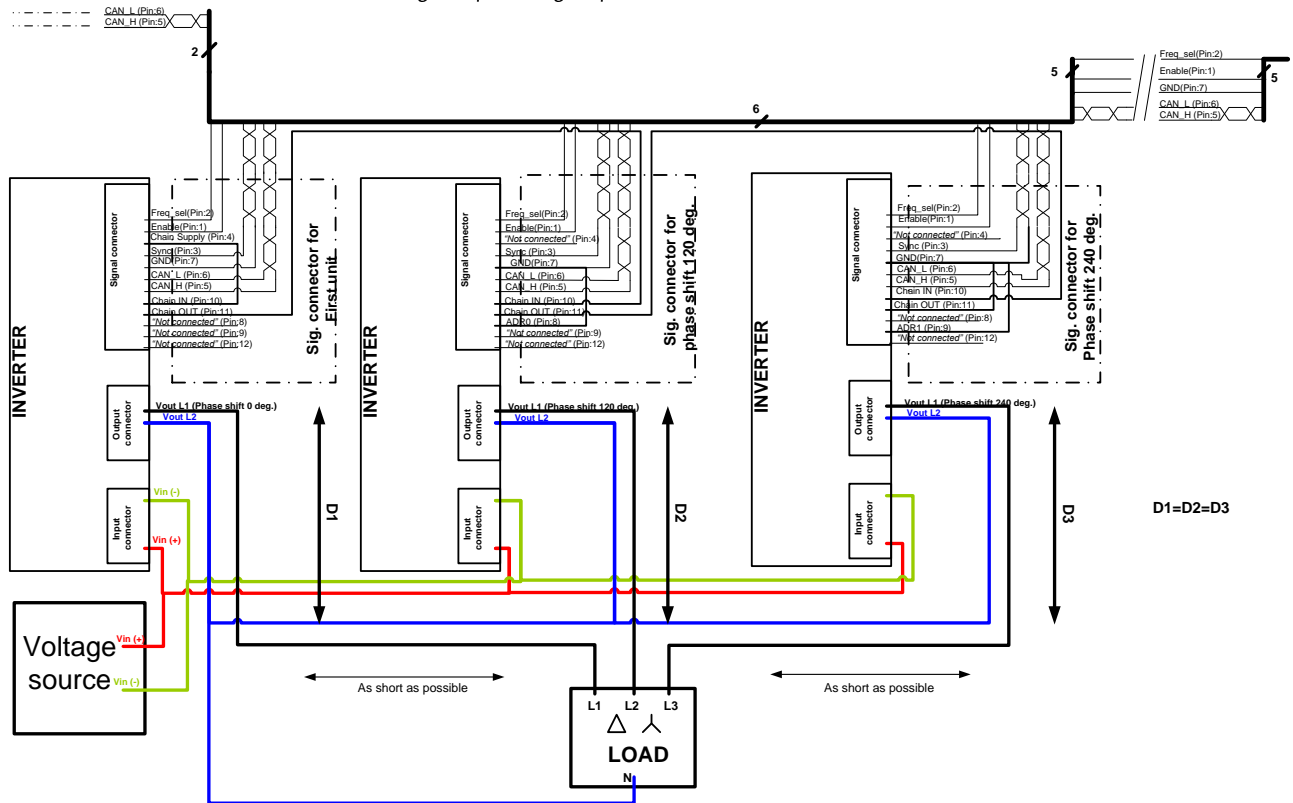
Wiring setup for 3-phase operation 700INV60-120-240-9G
