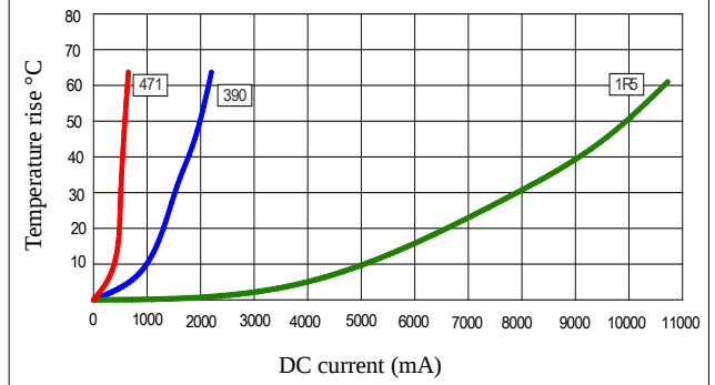
SCRH1035R Temperature rise by current
