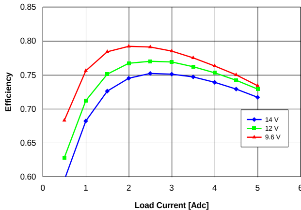
Fig. 1.0V.3: Efficiency vs. load current and input voltage for V_{out} = 1.0\text{ V} converter mounted vertically with air flowing at a rate of 200\text{ LFM} ( 1\text{ m/s} ) and T_a = 25\text{ }^{\circ}\text{C} .
