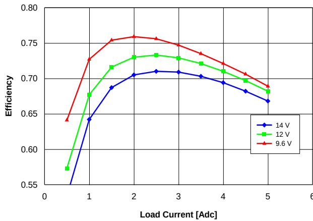
Fig. 0.7525V.3: Efficiency vs. load current and input voltage for V_{out} = 0.7525 V converter mounted vertically with air flowing at a rate of 200 LFM (1 m/s) and T_a = 25^\circ\text{C}
