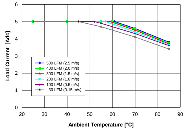
Fig. 1.5V.2: Available load current vs. ambient temperature and airflow rates for V_{out} = 1.5\text{ V} converter mounted horizontally with V_{in} = 12\text{ V} , and maximum MOSFET temperature \leq 120\text{ }^{\circ}\text{C} .
