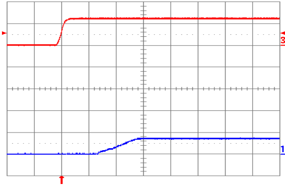
Fig. 0.7525V.5: Turn-on transient for V_{out} = 0.7525 V with application of V_{in} at full rated load current (resistive) and 100\ \mu\text{F} external capacitance at V_{in} = 12 V. Top trace: V_{in} (10 V/div.); Bottom trace: output voltage (1 V/div.); Time scale: 5 ms/div.
