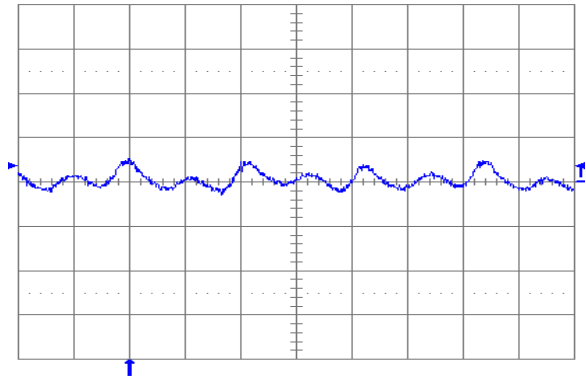
Fig. 1.5V.6: Output voltage ripple (20 mV/div.) at full rated load current into a resistive load with external capacitance 100\text{ }\mu\text{F} ceramic and V_{in} = 12\text{ V} for V_{out} = 1.5\text{ V} . Time scale: 1 \mu\text{s} /div.
