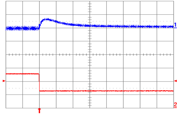
Fig. 1.2V.8: Output voltage response for V_{out} = 1.2\text{ V} to negative load current step change from 5\text{ A} to 2.5\text{ A} with slew rate of -5\text{ A}/\mu\text{s} at V_{in} = 12\text{ V} . Top trace: output voltage ( 100\text{ mV/div.} ); Bottom trace: load current ( 2\text{ A/div.} ). C_o = 100\text{ }\mu\text{F} ceramic. Time scale: 20\text{ }\mu\text{s/div.}
