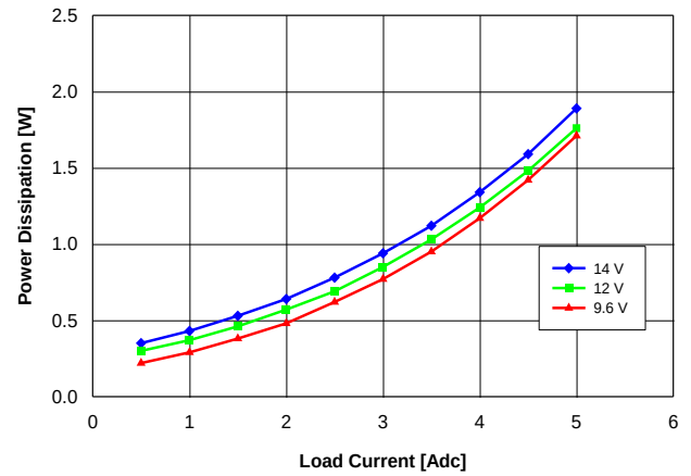
Fig. 0.7525V.4: Power Loss vs. load current and input voltage for V_{out} = 0.7525 V converter mounted vertically with air flowing at a rate of 200 LFM (1 m/s) and T_a = 25^\circ\text{C} .
