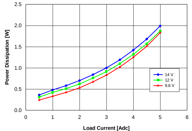
Fig. 1.0V.4: Power Loss vs. load current and input voltage for V_{out} = 1.0\text{ V} converter mounted vertically with air flowing at a rate of 200\text{ LFM} ( 1\text{ m/s} ) and T_a = 25\text{ }^{\circ}\text{C} .
