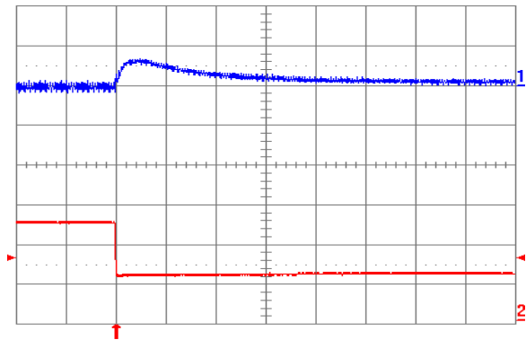
Fig. 0.7525V.8: Output voltage response for V_{out} = 0.7525 V to negative load current step change from 5 A to 2.5 A with slew rate of -5\ \text{A}/\mu\text{s} at V_{in} = 12 V. Top trace: output voltage (100 mV/div.); Bottom trace: load current (2 A/div.). C_o = 100\ \mu\text{F} ceramic. Time scale: 20\ \mu\text{s}/\text{div} .
