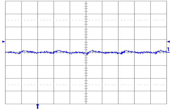
Fig. 0.7525V.6: Output voltage ripple (20 mV/div.) at full rated load current into a resistive load with external capacitance 100\ \mu\text{F} ceramic and V_{in} = 12 V for V_{out} = 0.7525 V. Time scale: 1\ \mu\text{s}/\text{div} .
