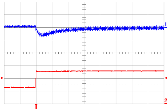
Fig. 0.7525V.7: Output voltage response for V_{out} = 0.7525 V to positive load current step change from 2.5 A to 5 A with slew rate of 5\ \text{A}/\mu\text{s} at V_{in} = 12 V. Top trace: output voltage (100 mV/div.); Bottom trace: load current (2 A/div.). C_o = 100\ \mu\text{F} ceramic. Time scale: 20\ \mu\text{s}/\text{div} .
