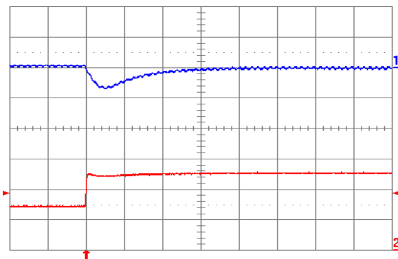
Fig. 0.7525V.7: Output voltage response for V_{out} = 0.7525V to positive load current step change from 2.5A to 5A with slew rate of 5A/\mu s at V_{in} = 5V . Top trace: output voltage (100mV/div.); Bottom trace: load current (2A/div.). C_o = 47\mu F ceramic. Time scale: 20µs/div.
