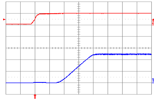
Fig. 2.5V.5: Turn-on transient for V_{out} = 2.5V with application of V_{in} at full rated load current (resistive) and 47\mu F external capacitance at V_{in} = 5V . Top trace: V_{in} (5V/div.); Bottom trace: output voltage (1V/div.); Time scale: 2ms/div.
