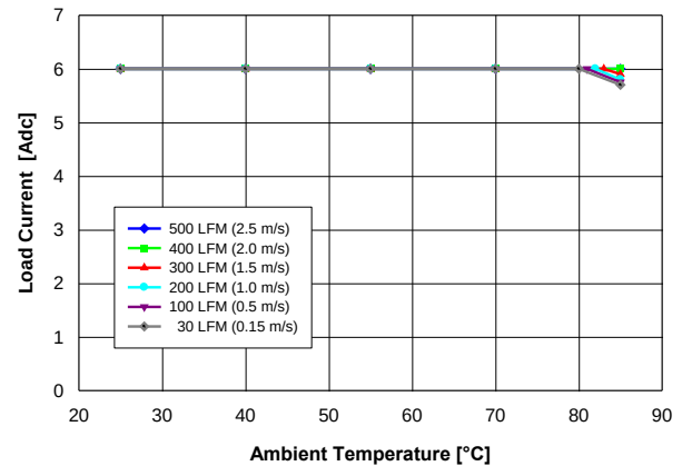
Fig. 1.0V.2: Available load current vs. ambient temperature and airflow rates for V_{out} = 1.0V converter mounted vertically or horizontally with V_{in} = 3.3V , air flowing from pin 5 to pin 1, and maximum MOSFET temperature \leq 120^\circ C .
