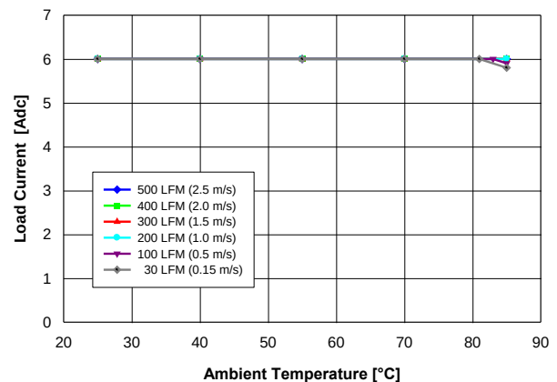
Fig. 0.7525V.2: Available load current vs. ambient temperature and airflow rates for V_{out} = 0.7525V converter mounted vertically or horizontally with V_{in} = 3.3V , air flowing from pin 5 to pin 1, and maximum MOSFET temperature \leq 120^\circ C .
