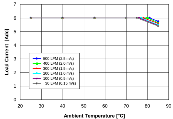
Fig. 3.3V.2: Available load current vs. ambient temperature and airflow rates for V_{out} = 3.3\text{V} converter mounted horizontally with V_{in} = 5\text{V} , air flowing from pin 1 to pin 5, and maximum MOSFET temperature \leq 120^\circ\text{C} .
