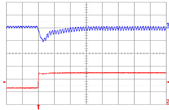
Fig. 1.5V.7: Output voltage response for V_{out} = 1.5V to positive load current step change from 2.5A to 5A with slew rate of 5A/\mu s at V_{in} = 5V . Top trace: output voltage (100mV/div.); Bottom trace: load current (2A/div.). C_o = 47\mu F ceramic. Time scale: 20µs/div.
