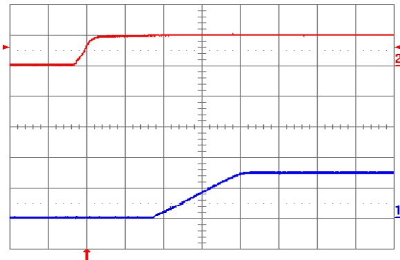
Fig. 0.7525V.5: Turn-on transient for V_{out} = 0.7525V with application of V_{in} at full rated load current (resistive) and 47\mu F external capacitance at V_{in} = 5V . Top trace: V_{in} (5V/div.); Bottom trace: output voltage (1V/div.); Time scale: 2ms/div.
