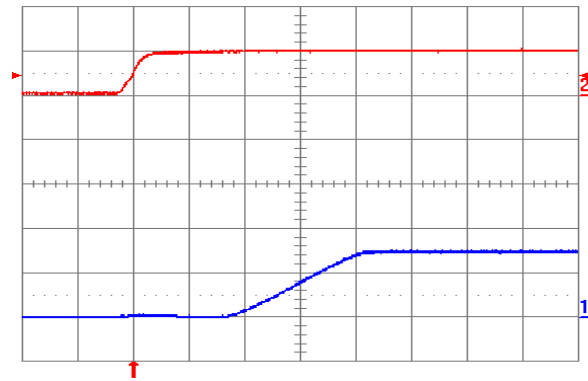
Fig. 1.5V.5: Turn-on transient for V_{out} = 1.5V with application of V_{in} at full rated load current (resistive) and 47\mu F external capacitance at V_{in} = 5V . Top trace: V_{in} (5V/div.); Bottom trace: output voltage (1V/div.); Time scale: 2ms/div.
