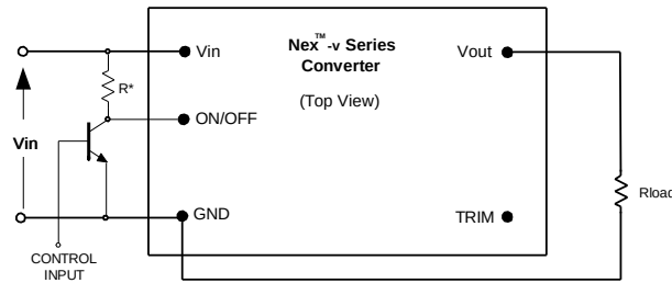
Fig. C: Circuit configuration for ON/OFF function.
