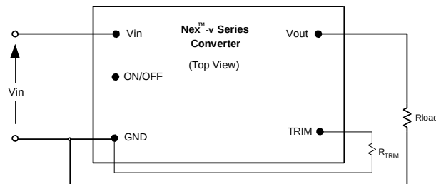
Fig. D: Configuration for programming output voltage
