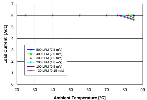
Fig. 1.5V.2: Available load current vs. ambient temperature and airflow rates for V_{out} = 1.5V converter mounted vertically or horizontally with V_{in} = 3.3V , air flowing from pin 5 to pin 1, and maximum MOSFET temperature \leq 120^\circ C .
