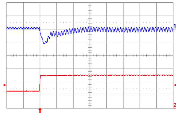
Fig. 2.5V.7: Output voltage response for V_{out} = 2.5V to positive load current step change from 2.5A to 5A with slew rate of 5A/\mu s at V_{in} = 5V . Top trace: output voltage (100mV/div.); Bottom trace: load current (2A/div.). C_o = 47\mu F ceramic. Time scale: 20µs/div.
