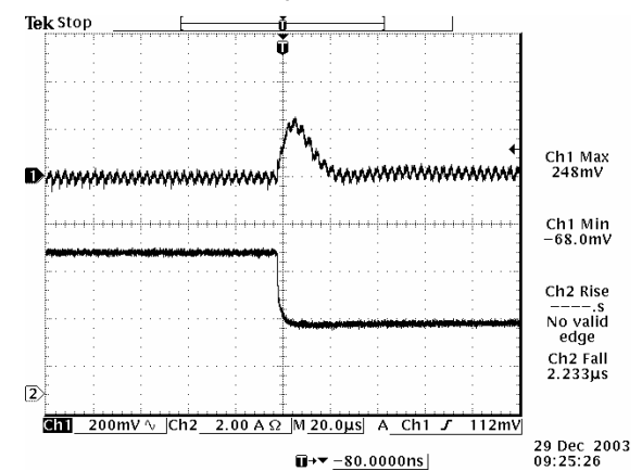
100% to 50% load step at V_{in}=12 V, V_o=5.0 V
