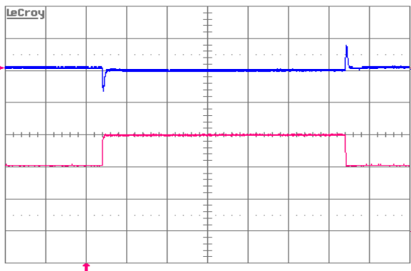
Figure 9. Output voltage response to load current step-change (20 A – 30 A – 20 A) at V_{in} = 48\text{ V} . Top trace: output voltage (200 mV/div.). Bottom trace: load current (10 A/div.). Current slew rate: 2.5 A/ \mu\text{s} . C_o = 470\text{ }\mu\text{F} POS + 1 \mu\text{F} ceramic. Time scale: 0.2 ms/div.
