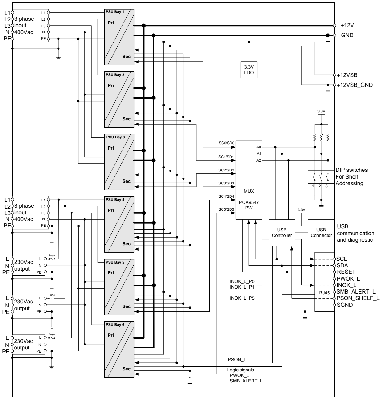
Figure 1. SPSPF3-04G Block Diagram
