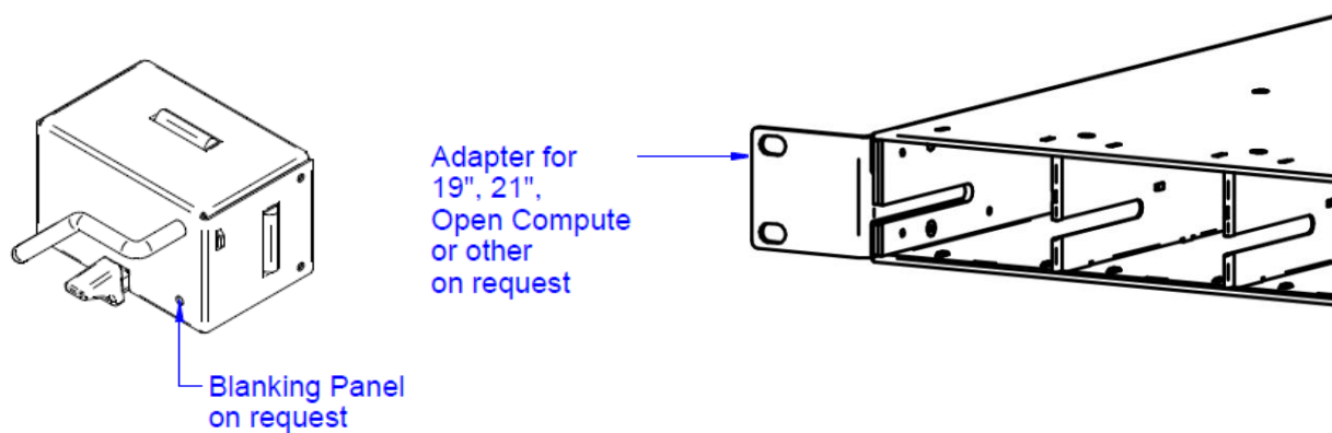
Figure 9. Accessories
