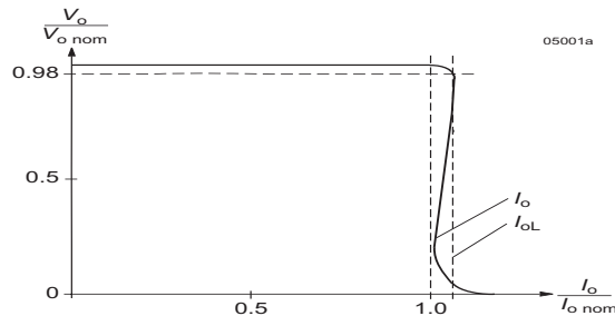
Fig. 12 Typ output characteristic V_{o1} versus I_{o1} .
