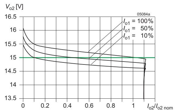
Fig. 15 LS5540: V_{o2} versus I_{o2} with various I_{o1} (typ).
