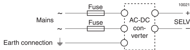
Fig. 12 Schematic safety concept
