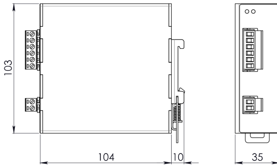
Figure 1. Mechanical Drawing
