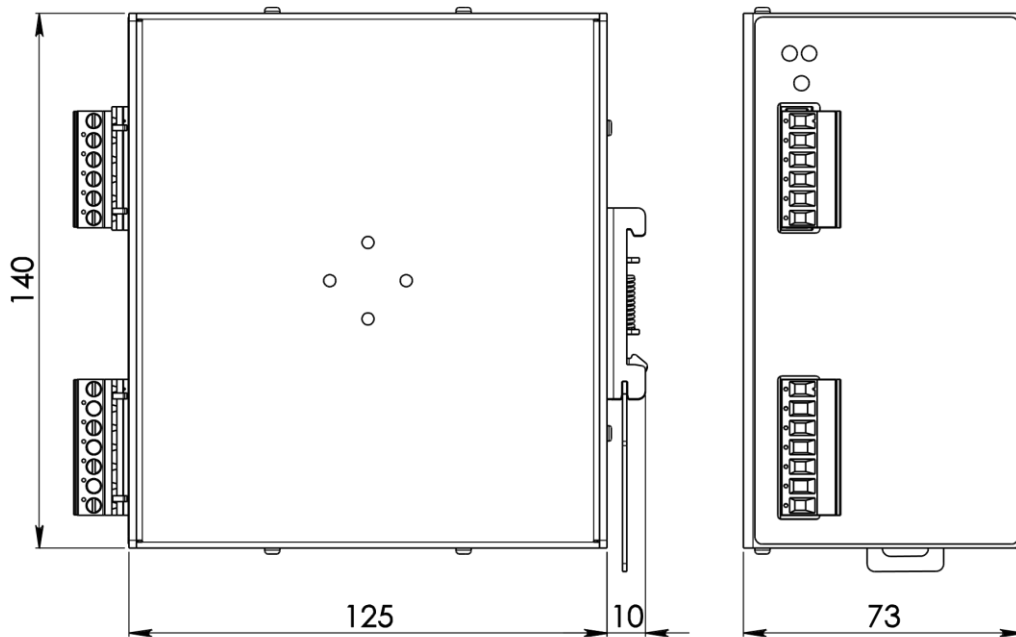
Figure 1. Mechanical Drawing
