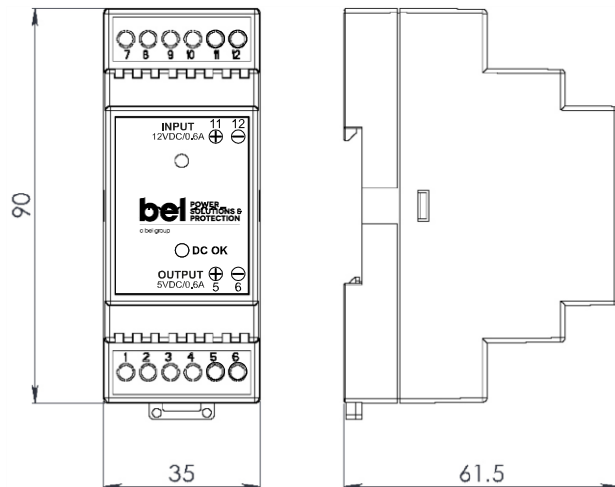
Figure 1. Mechanical Drawing
