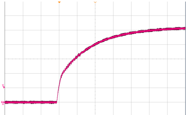
Figure 11. Rise time V_{BC} at 277VAC, 2A load (50ms/div) CH4: V_{BC} (10V/div)
