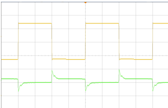
Figure 12. Load transient V_1 , 133A to 265A, 1A/μs (5ms/div) CH1: I_1 (50A/div) CH2: V_1 (500mV/div)
