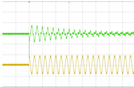
Figure 4. Inrush current, V_{in} = 290\ VAC, 90^\circ CH1: V_{in} (500 V/div), CH2: I_{in} (10 A/div)
