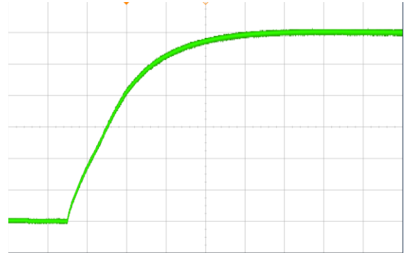
Figure 9. Rise time V_1 at 277VAC, full load (500μs/div) CH2: V_1 (2V/div)
