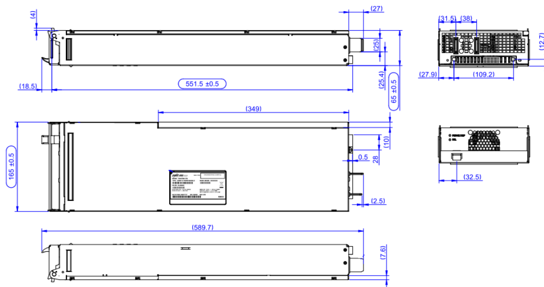
Figure 24. Mechanical Drawing
