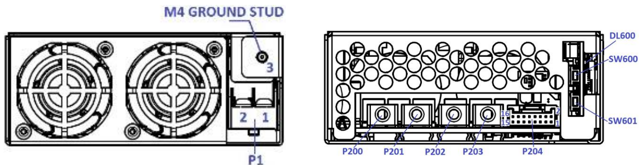
Figure 9. Rear View - ABE1200-1T24 / ABE1200-1T48 Models
