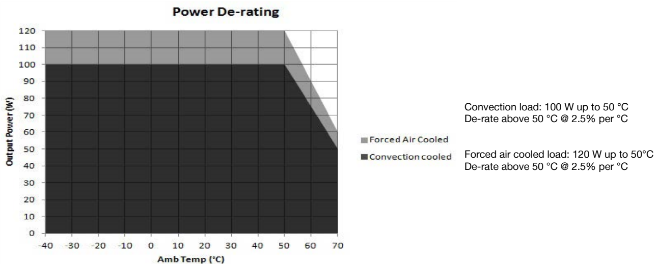
Figure 1. Derating Curve
