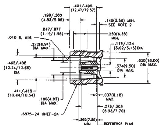
Female Jack
