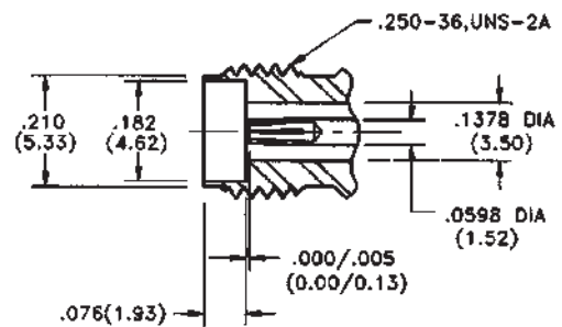
Female Jack
