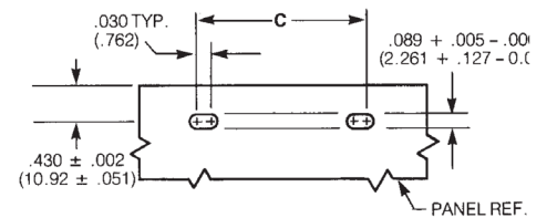
Figure 3: Edgeboard Mounting
