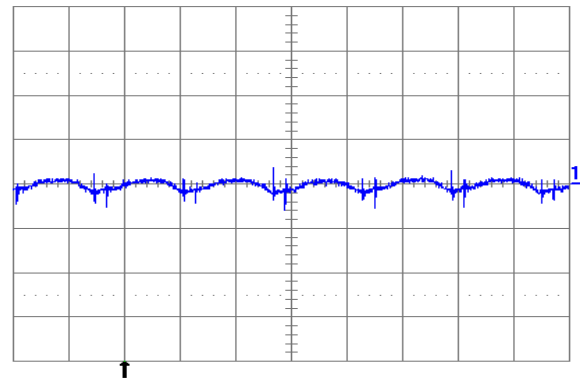
Fig. 1.5V.6: Output voltage ripple (20mV/div.) at full rated load current into a resistive load with external capacitance 100\mu F ceramic and V_{in} = 12V for V_{out} = 1.5V . Time scale: 2µs/div.
