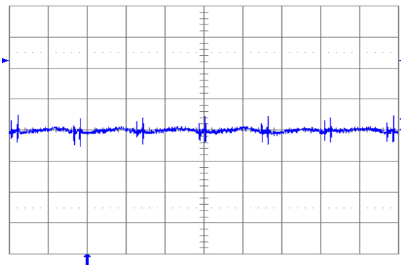
Fig. 1.0V.6: Output voltage ripple (20mV/div.) at full rated load current into a resistive load with external capacitance 100\mu F ceramic and V_{in} = 12V for V_{out} = 1.0V . Time scale: 2\mu s /div.
