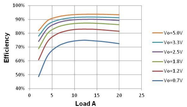
Figure 8. Efficiency vs Load, V_{in}=12\text{ V} , F_{sw}=500\text{ KHz}
