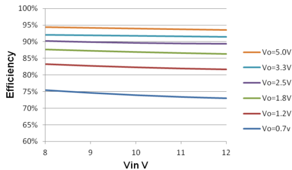
Figure 7. Efficiency vs. Input Voltage, I_{out}=20\text{ A} , F_{sw}=500\text{ KHz}
