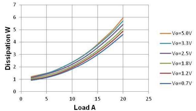
Figure 6. Dissipation vs Load, V_{in}=8\text{ V} , F_{sw}=500\text{ KHz}
