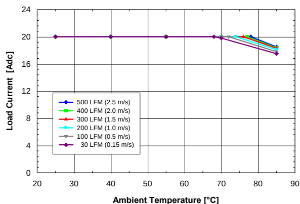
Figure 1. Available output current vs. ambient air temperature and airflow rates for converter DP8120G mounted horizontally with air flowing from input to output, MOSFET temperature \leq 120^{\circ}\text{C} , V_{in} = 8\text{ V} , V_{out} = 5\text{ V} , and F_{sw} = 500\text{KHz}
