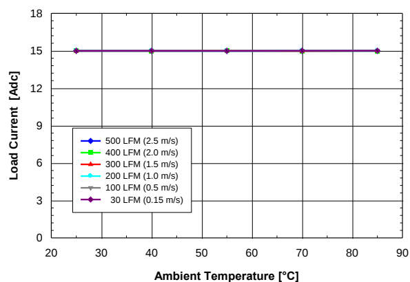
Figure 2. Available output current vs. ambient air temperature and airflow rates for converter DP8120G mounted horizontally with air flowing from input to output, MOSFET temperature \leq 120^{\circ}\text{C} , V_{in} = 8\text{ V} , V_{out} = 5\text{ V} , and F_{sw} = 1\text{MHz}
