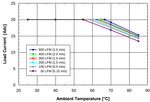
Figure 3. Available output current vs. ambient air temperature and airflow rates for converter DP8120G mounted horizontally with air flowing from input to output, MOSFET temperature 120°C, V_{in} = 12\text{ V} , V_{out} = 5\text{ V} , and F_{sw} = 500\text{ KHz}
