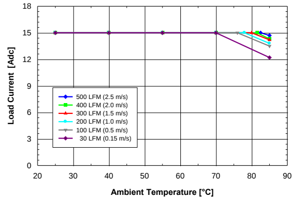
Figure 4. Available output current vs. ambient air temperature and airflow rates for converter DP8120G mounted horizontally with air flowing from input to output, MOSFET temperature 120°C, V_{in} = 12\text{ V} , V_{out} = 5\text{ V} , and F_{sw} = 1\text{ MHz}
