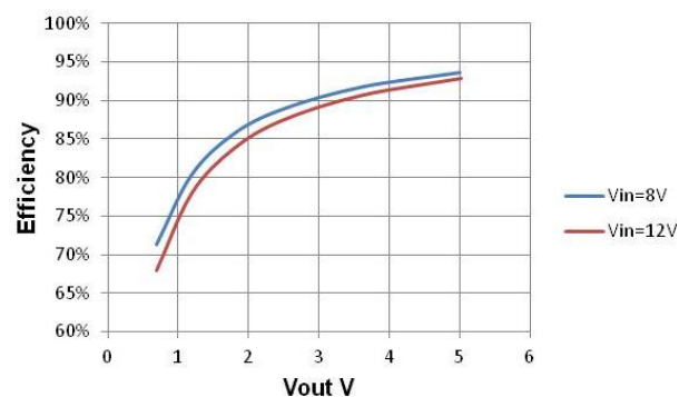
Figure 12. Efficiency vs V_{out} , I_{out}=20A , F_{sw}=1MHz
