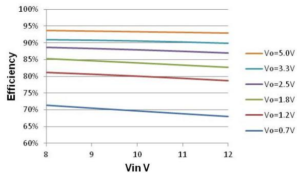
Figure 10. Efficiency vs V_{in} , I_{out}=20A , F_{sw}=1MHz
