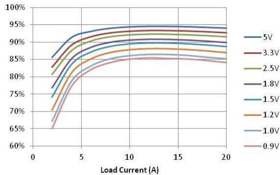
Figure 5. Efficiency vs. Load, V_{in}=8\text{ V} , F_{sw}=500\text{ KHz}
