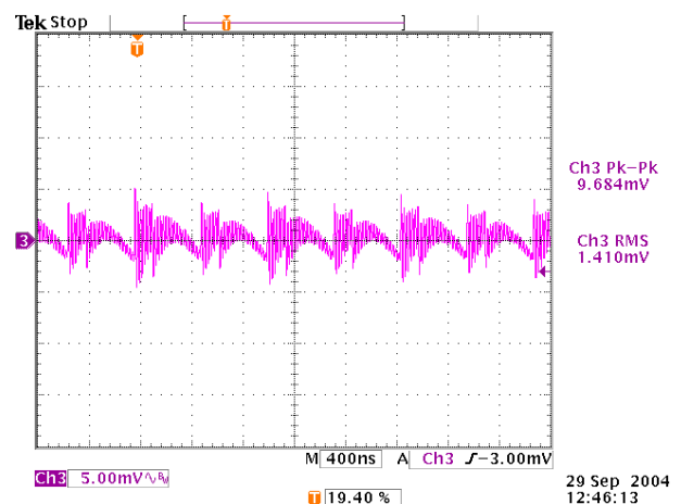
Figure 48. Output Voltage Noise, Full Load, 180° Interleave
