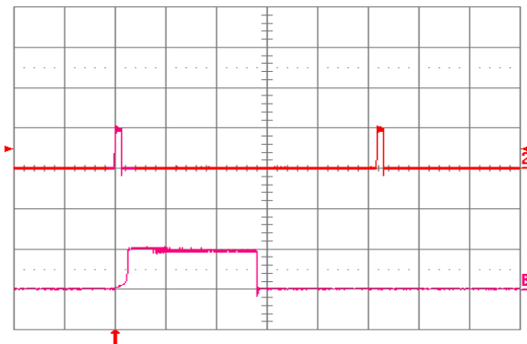
Fig. 3.3V.18: Load current (top trace, 20 A/div., 20 ms/div.) into a 10 \text{ m}\Omega short circuit during restart, at V_{in} = 24 \text{ V} . Bottom trace (20 A/div., 1 ms/div.) is an expansion of the on-time portion of the top trace.
