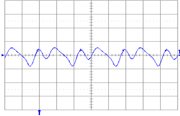
Fig. 1.0V.13: Output voltage ripple (20 mV/div.) at full rated load current into a resistive load with C_o = 10 \mu\text{F} tantalum + 1\mu\text{F} ceramic and V_{in} = 24 \text{ V} . Time scale: 1 \mu\text{s}/\text{div} .
