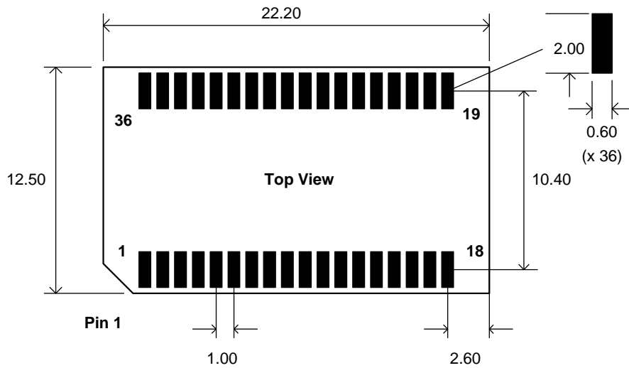
Figure 54. Recommended PCB Pad Sizes
