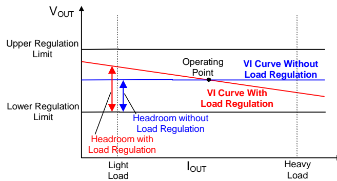
Figure 8 Optimal Voltage Positioning Concept
