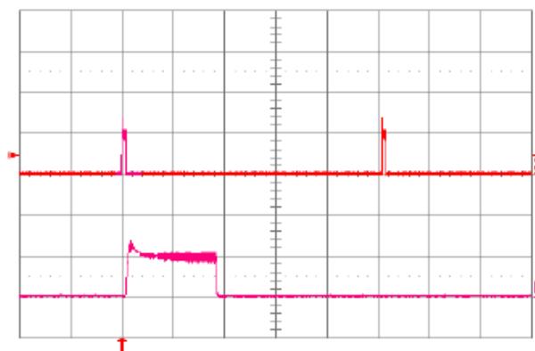
Fig. 12V.18: Load current (top trace, 5A/div., 20 ms/div.) into a 10 m \Omega short circuit during restart, at V_{in} = 48V . Bottom trace (5A/div., 1ms/div.) is an expansion of the on-time portion of the top trace.
