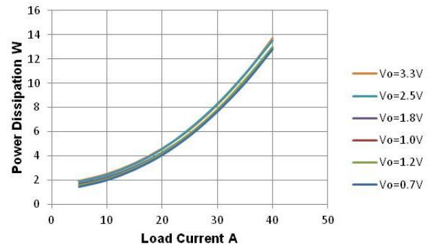
Figure 4. Dissipation vs Load, V_{in}=8V , F_{sw}=500kHz
