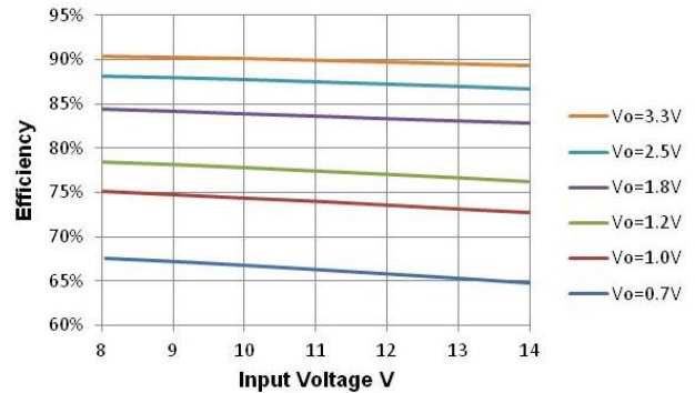
Figure 6. Efficiency vs V_{in} , Load=40A, F_{sw}=500kHz
