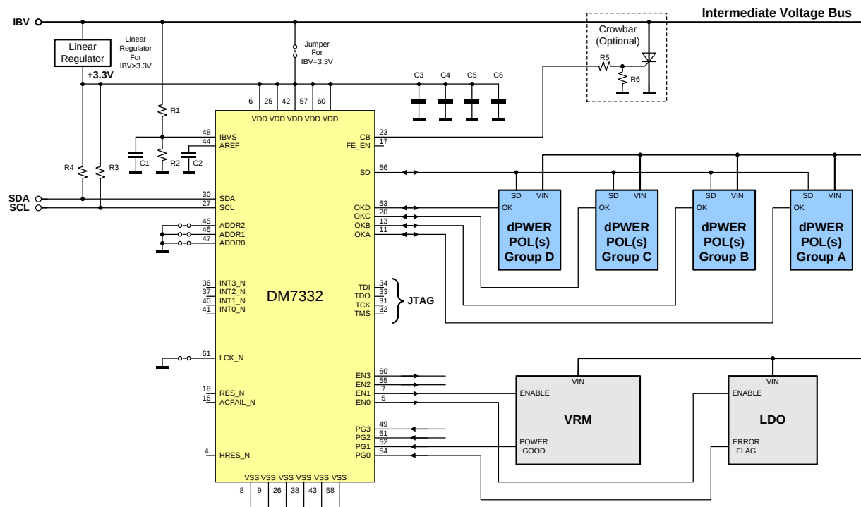
Figure 50. Multi-dPOL Power System Diagram
