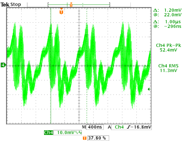
Figure 39. Input Voltage Noise, No Interleave
