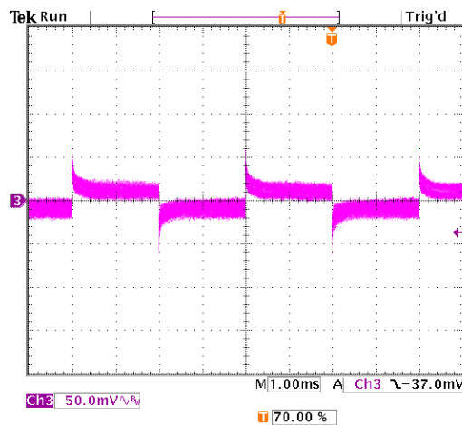
Figure 45. Transient Response with Regulation set to 0.55mV/A
