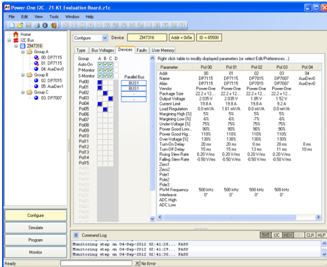
Figure 47 Evaluation Board Configuration showing Current Share Bus Assignment
