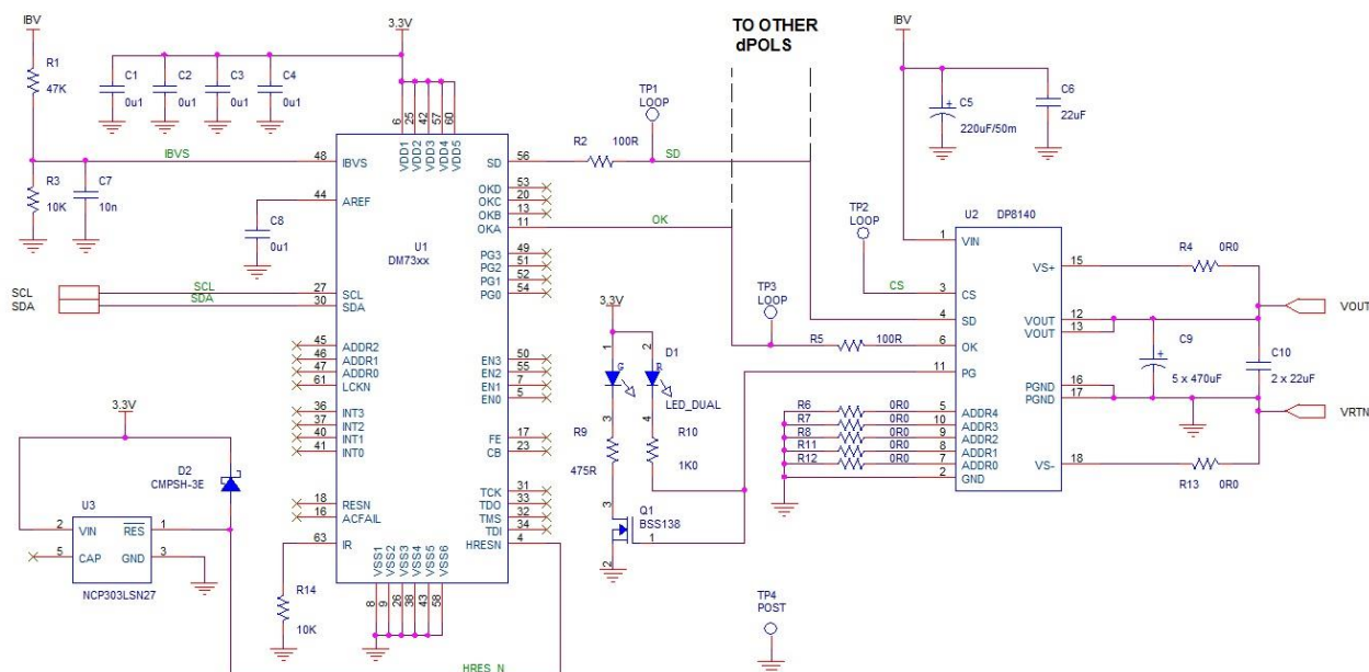
Figure 51. Typical Application with Digital Power Manager and I2C Interface
