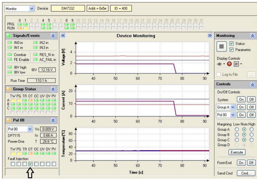
Figure 49. Example Overtemp Fault Injection in the GUI
