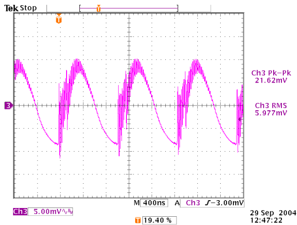
Figure 41. Output Voltage Noise, Full Load, No Interleave
