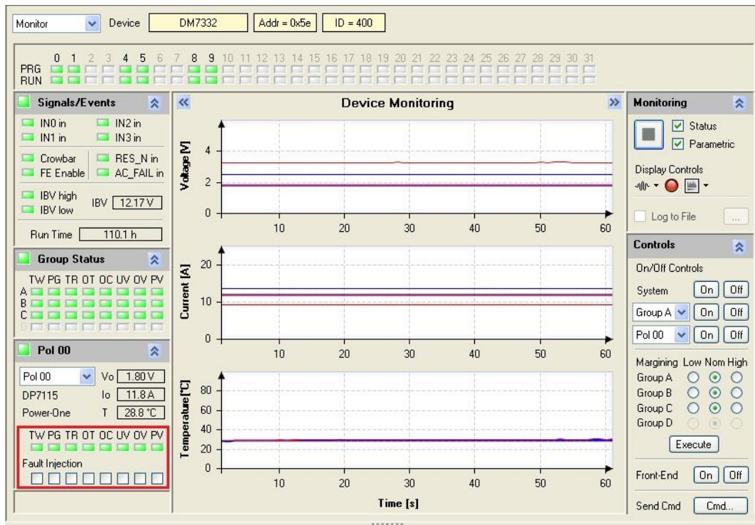
Figure 48. Fault Injection Controls In Monitor Window
