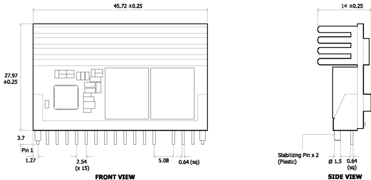
Figure 52. Mechanical Drawing
