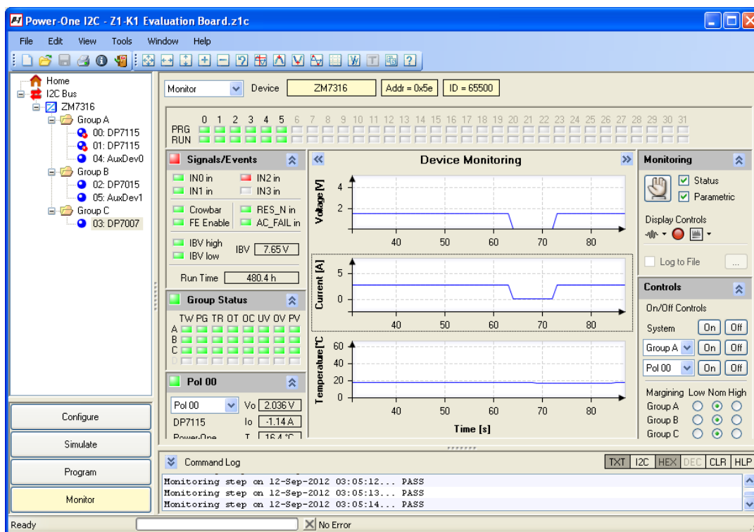
Figure 46. DPM Monitoring Window
