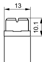
Fig. 12 HZZ00116 (STV-H15 S2-FSF/CO) 11 faston terminals and two screw jacks. HZZ00115 (STV-H15 S2-F/CO) 11 faston terminals and two solder jacks (solder jacks are shown in fig. 15).
