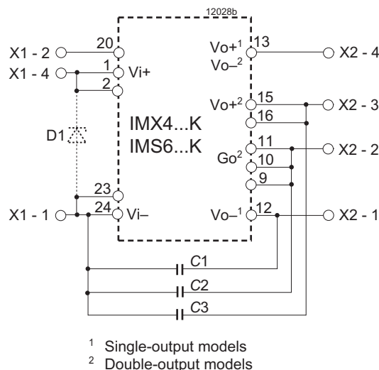
Fig. 14 Circuit diagram of CMB3W and DMB3W
