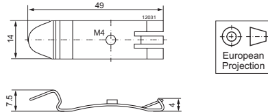
Fig. 4 DIN-rail clamp XMM162-G, steel, galvanized
