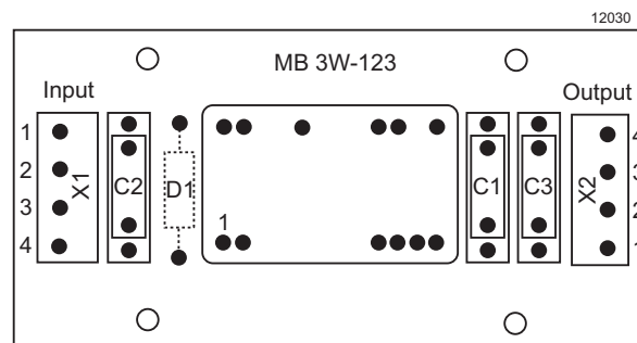
Fig. 15 Print layout of CMB3W and DMB3W
