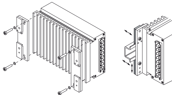
Fig. 9a Schematic view: Assembly of HZZ00615-G (DMB-K/S)
