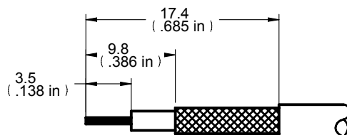
CABLE STRIP DIMENSIONS
