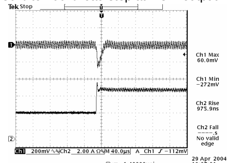
50% to 100% load step at 3.3 V output
