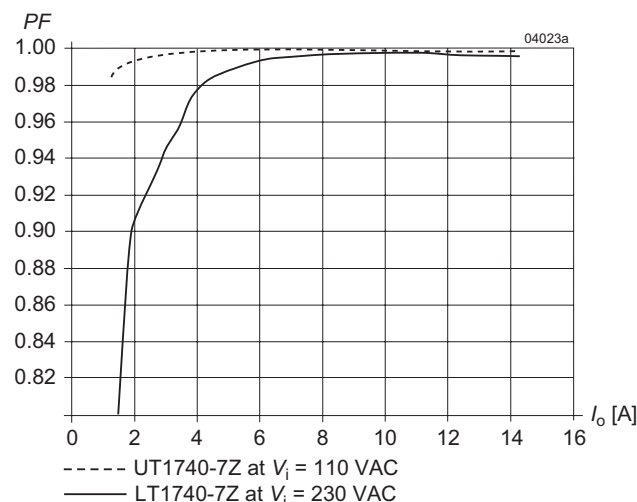
Fig. 2 Power factor
