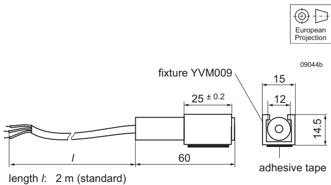
Fig. 57 Mechanical dimensions (in mm)
