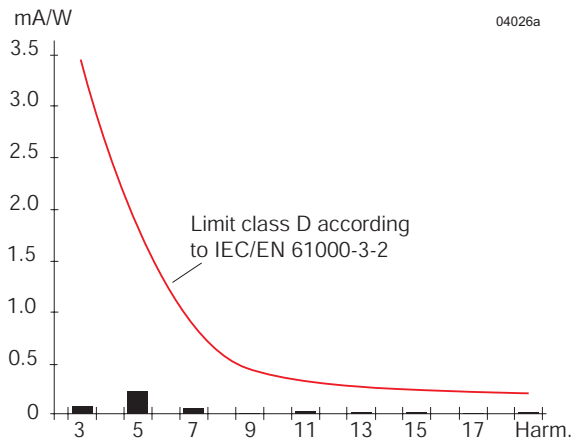
Fig. 3 Harmonic distortion at input LT1740-7Z, V_i = V_{i nom} , I_o = I_{o nom}
