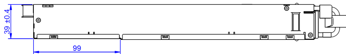
Figure 37. Side View 2
