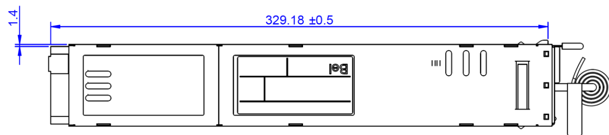
Figure 36. Top View
