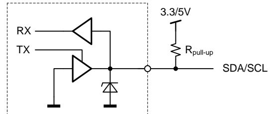
Figure 10. Physical layer of communication interface
