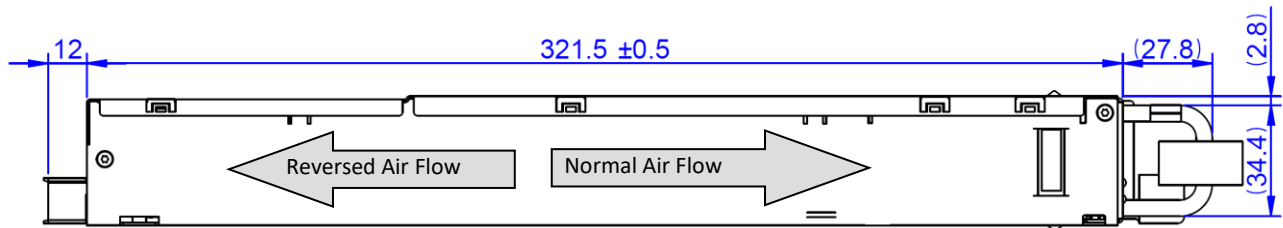
Figure 14 Side View 1
