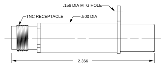
PATCH JACK TNC
