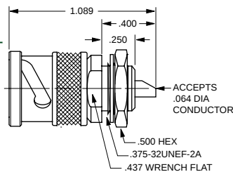
BULKHEAD PLUG FRONT MOUNT, SOLDER POT
