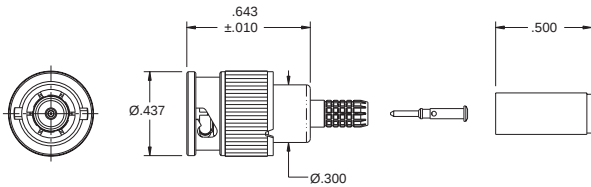
MINIATURE BNC (M-BNC) COAXIAL PLUG STRAIGHT 75Ω UPL250-1
