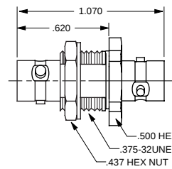
FEED-THROUGH JACK
