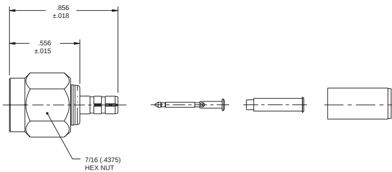
75 OHM "F" TYPE TOOL CRIMP PLUG PL130SC- (see dash number from chart on right)
