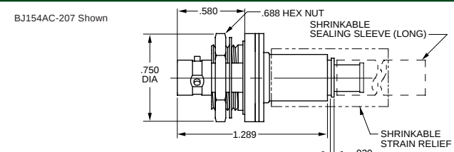
INSULATED BULKHEAD JACK REAR MOUNT, TOOL CRIMP
