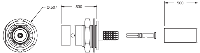
MINIATURE BNC (M-BNC) COAXIAL BULKHEAD JACK STRAIGHT 75Ω UBJ250-1
