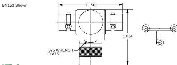
"T" ADAPTER
