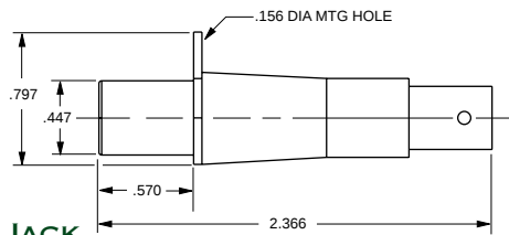
PATCH JACK BNC REAR INTERFACE
