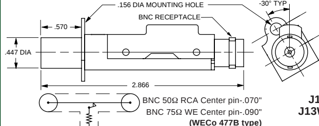
PATCH JACK SELF-TERMINATING
