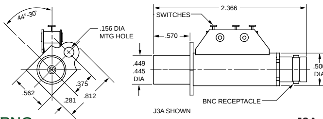
BNC PATCH JACK
