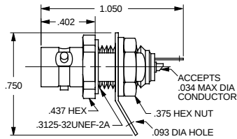
BULKHEAD JACK FRONT MOUNT, SOLDER POT
