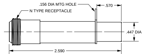
PATCH JACK "N"
