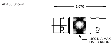
TRS/TTM COUPLING ADAPTER (BARREL CONNECTOR)
