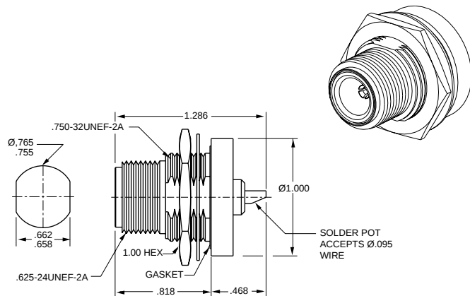
"N" TYPE BULKHEAD JACK
