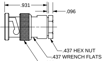
CABLE PLUG WRENCH CRIMP
