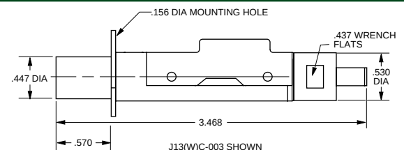
PATCH JACK SELF-TERMINATING
