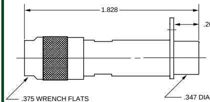
MINIATURE PATCH JACK CABLE ENTRY, FIELD SERVICEABLE MINI-WECO TYPE Minimum .64" centers
