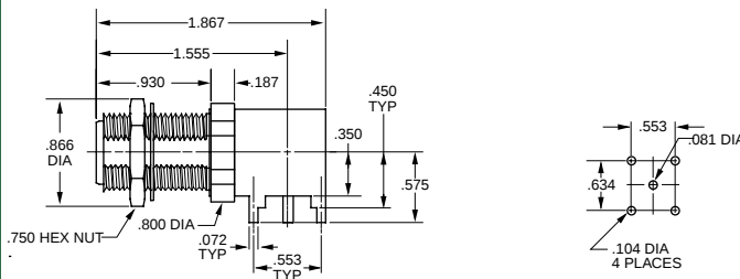
RIGHT ANGLE CIRCUIT BOARD JACK
