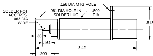
PATCH JACK SOLDER POT
