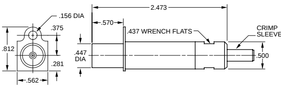
PATCH JACK CRIMP
