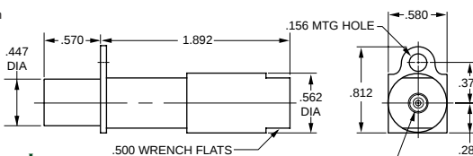
PATCH JACK CABLE ENTRY
