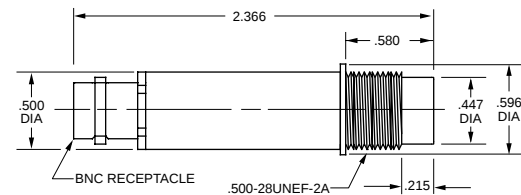
PATCH JACK BNC
