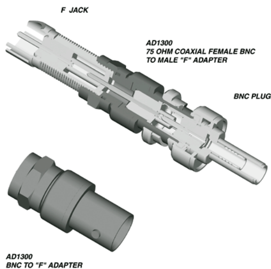
F ADAPTER
