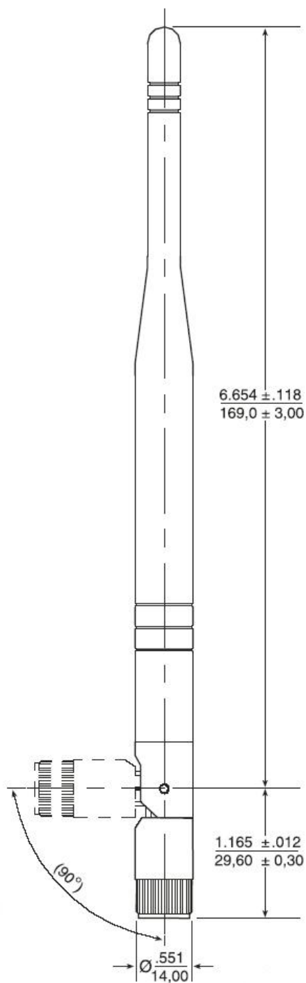
ZXT9-RM Antenna
