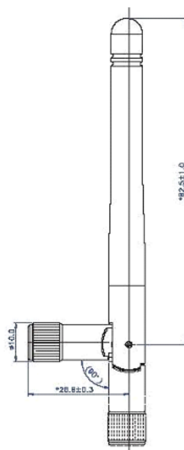
ZXT24-RM Antenna
